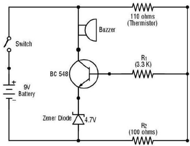
Fig.8. Fire alarm circuit
